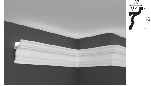
KH 916 62 x 37 mm
