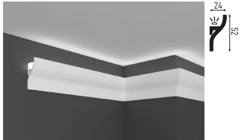
KH 906 (F) 52 x 24 mm
