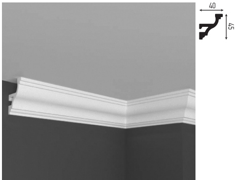
KH 905 (F) 45 x 40 mm
